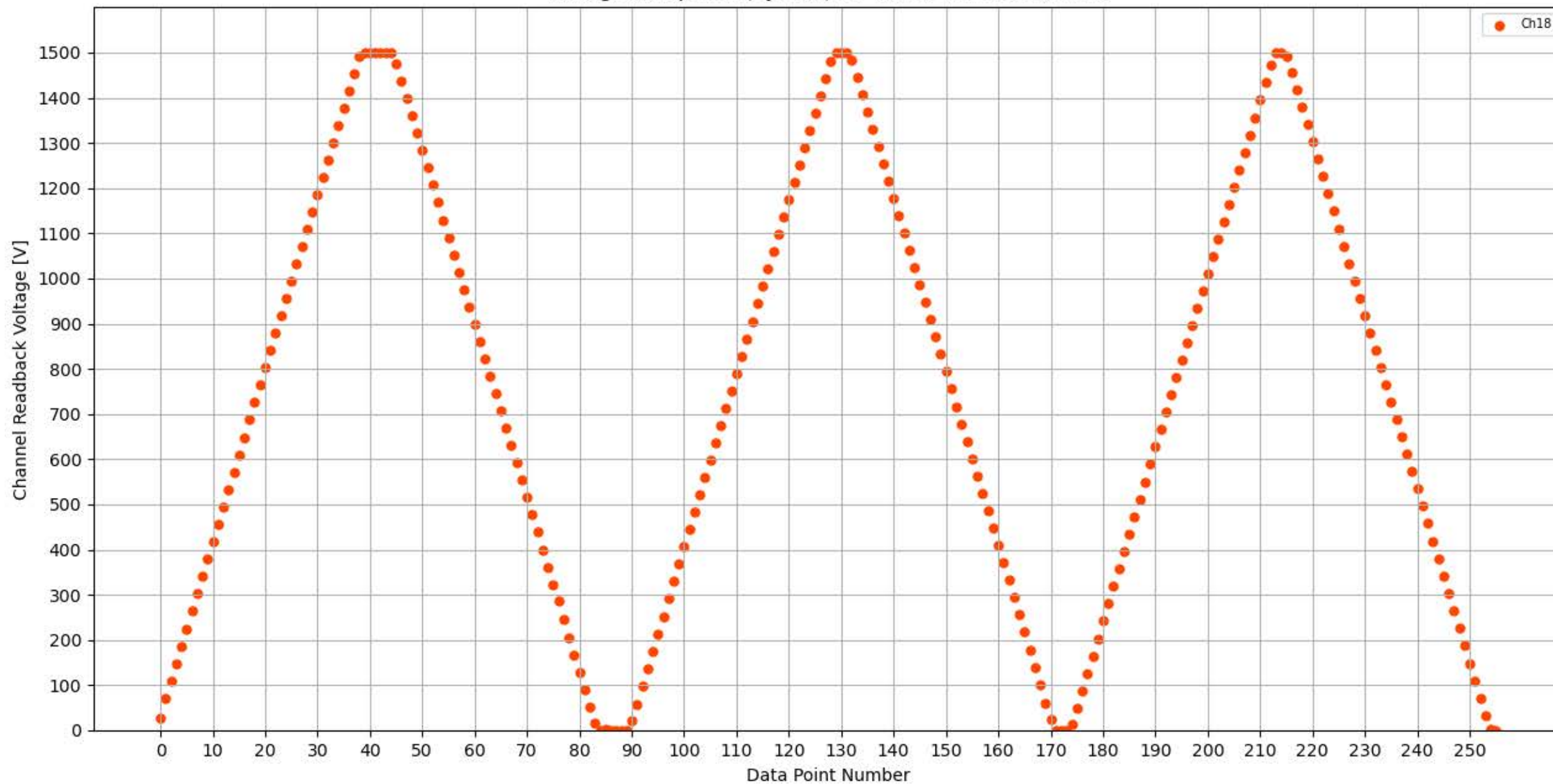
Voltage Ramp Test (Python) Bd #313, Slot #8, Ch #18
