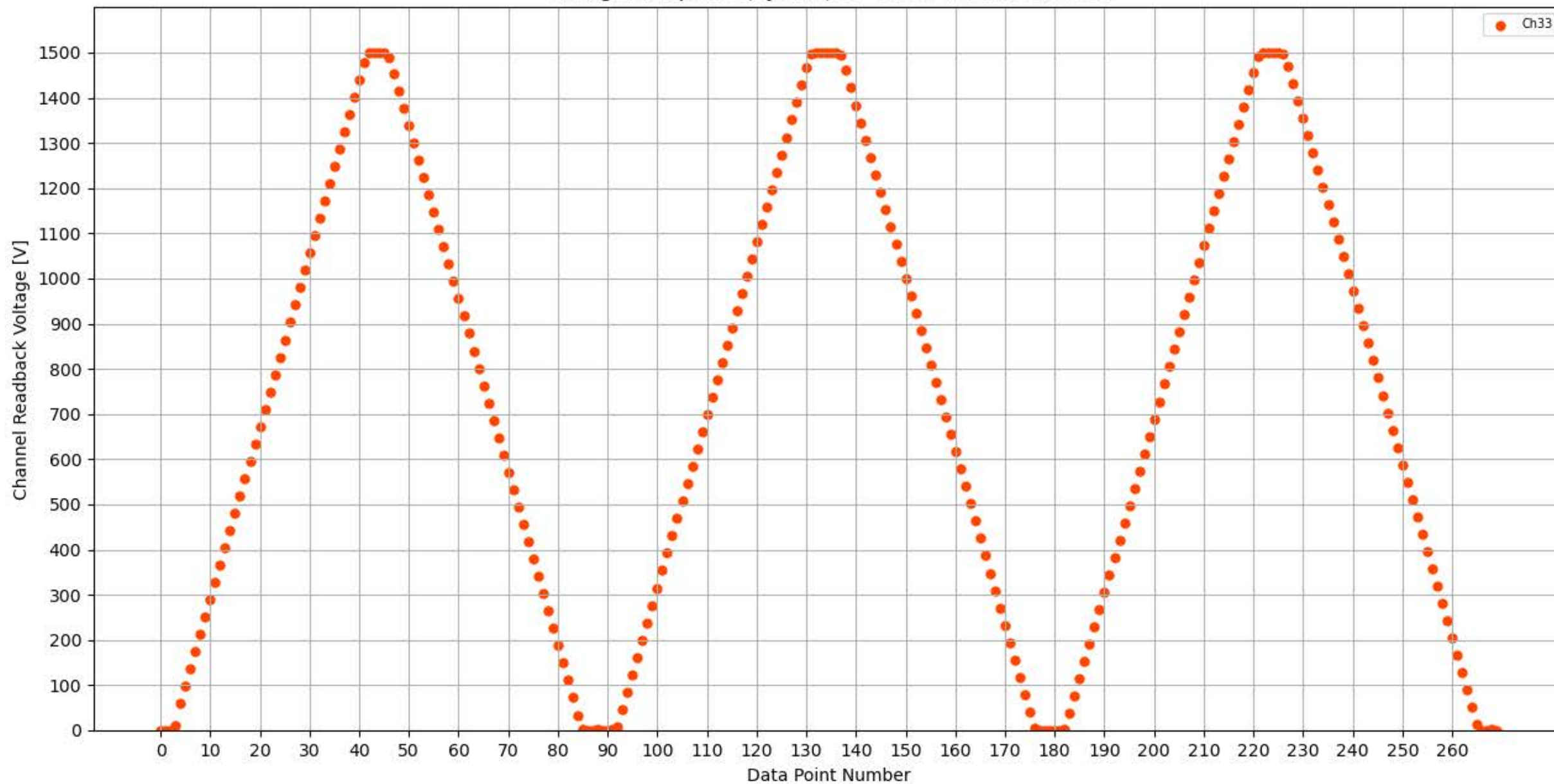
Voltage Ramp Test (Python) Bd #313, Slot #8, Ch #33
