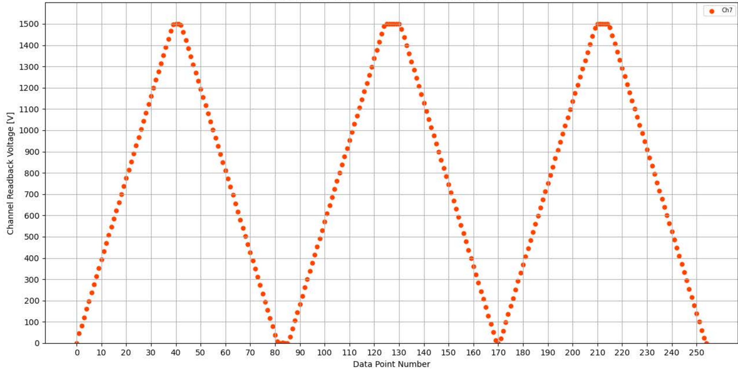
Voltage Ramp Test (Python) Bd #313, Slot #8, Ch #7
