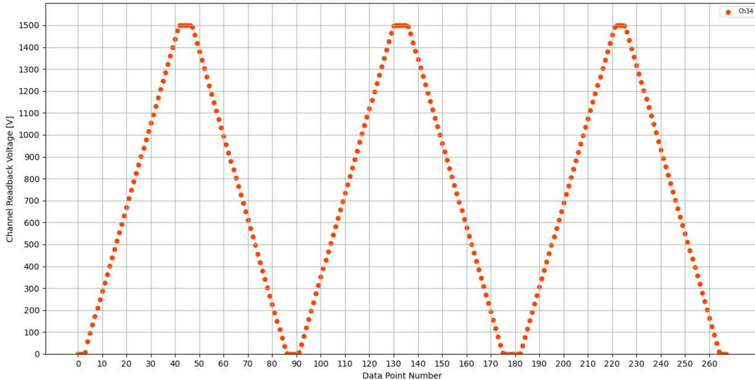
Voltage Ramp Test (Python) Bd #313, Slot #8, Ch #34
