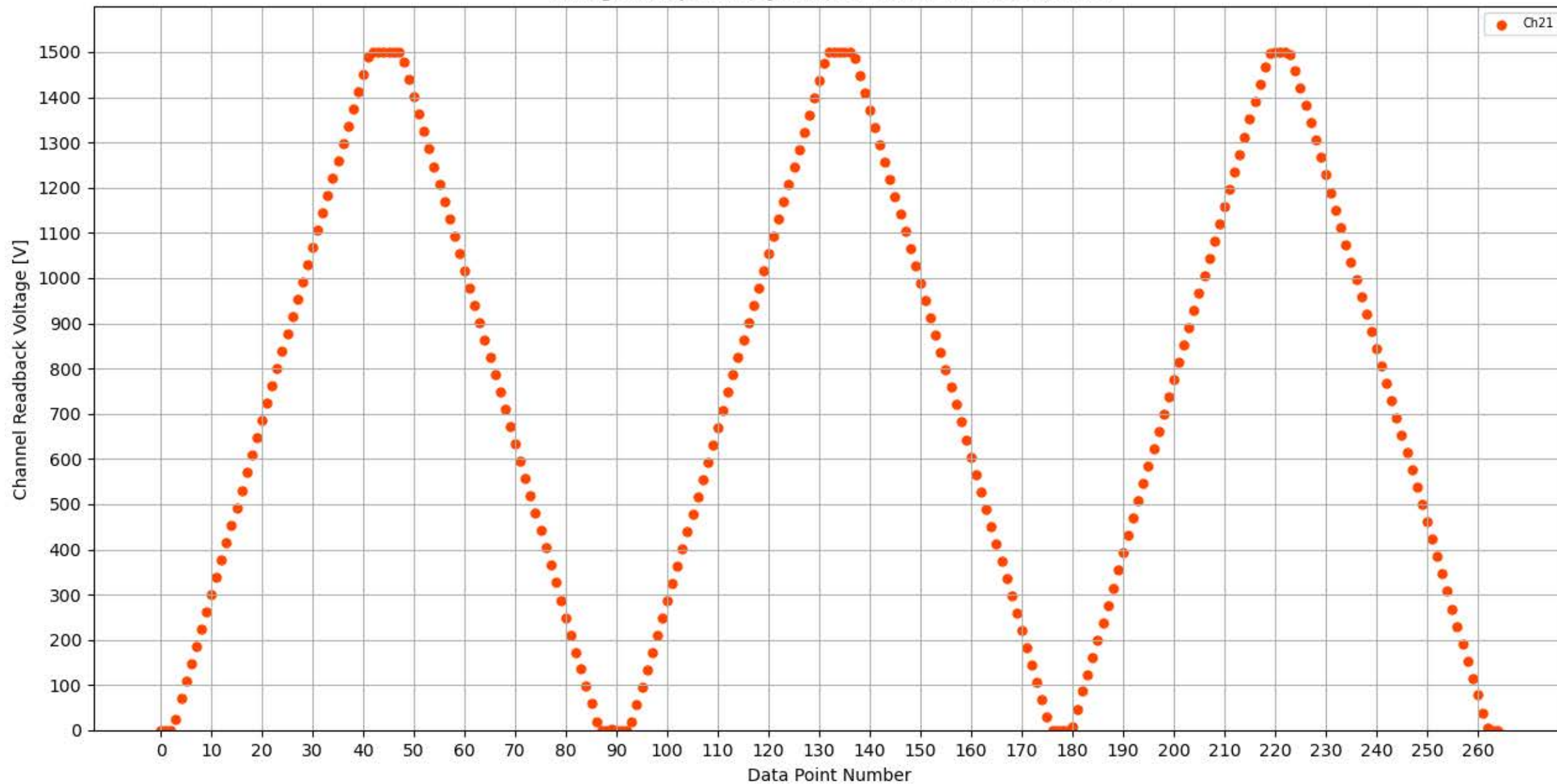
Voltage Ramp Test (Python) Bd #313, Slot #8, Ch #21
