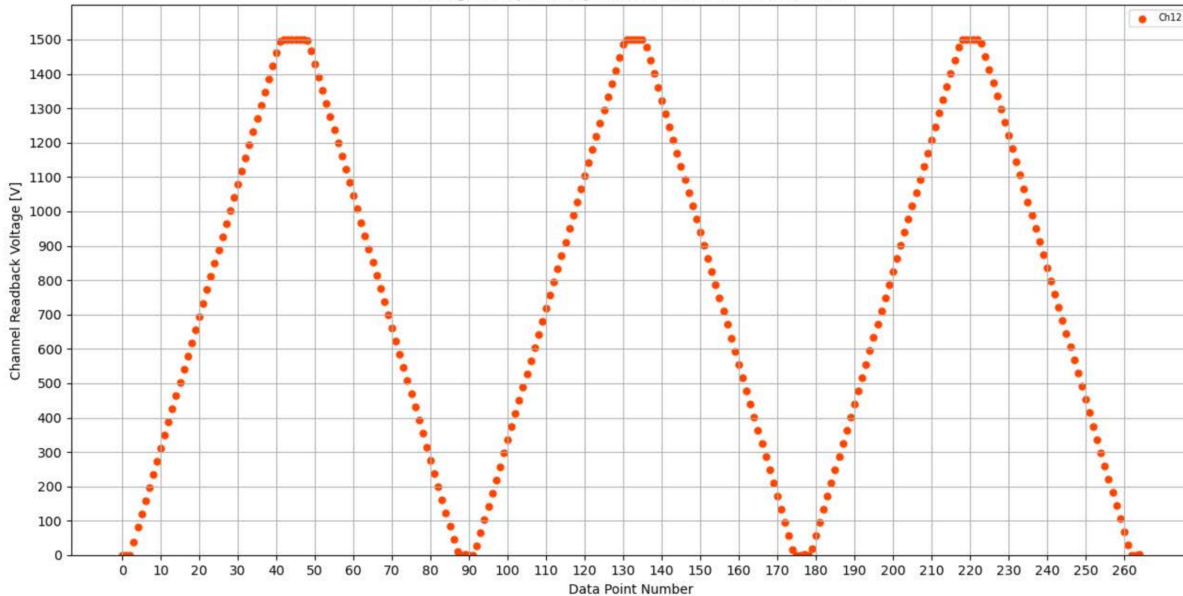
Voltage Ramp Test (Python) Bd #313, Slot #8, Ch #12
