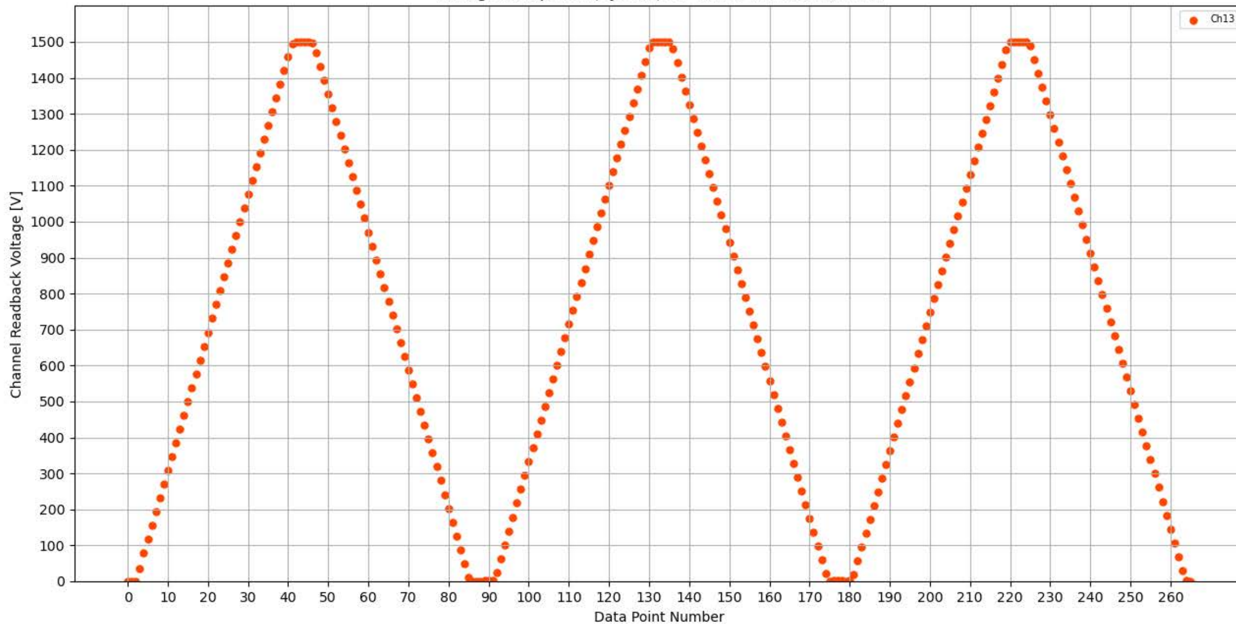
Voltage Ramp Test (Python) Bd #313, Slot #8, Ch #13
