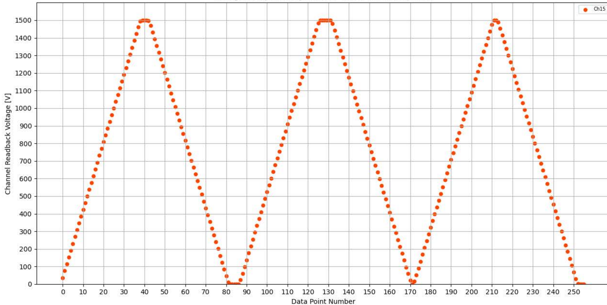
Voltage Ramp Test (Python) Bd #313, Slot #8, Ch #15
