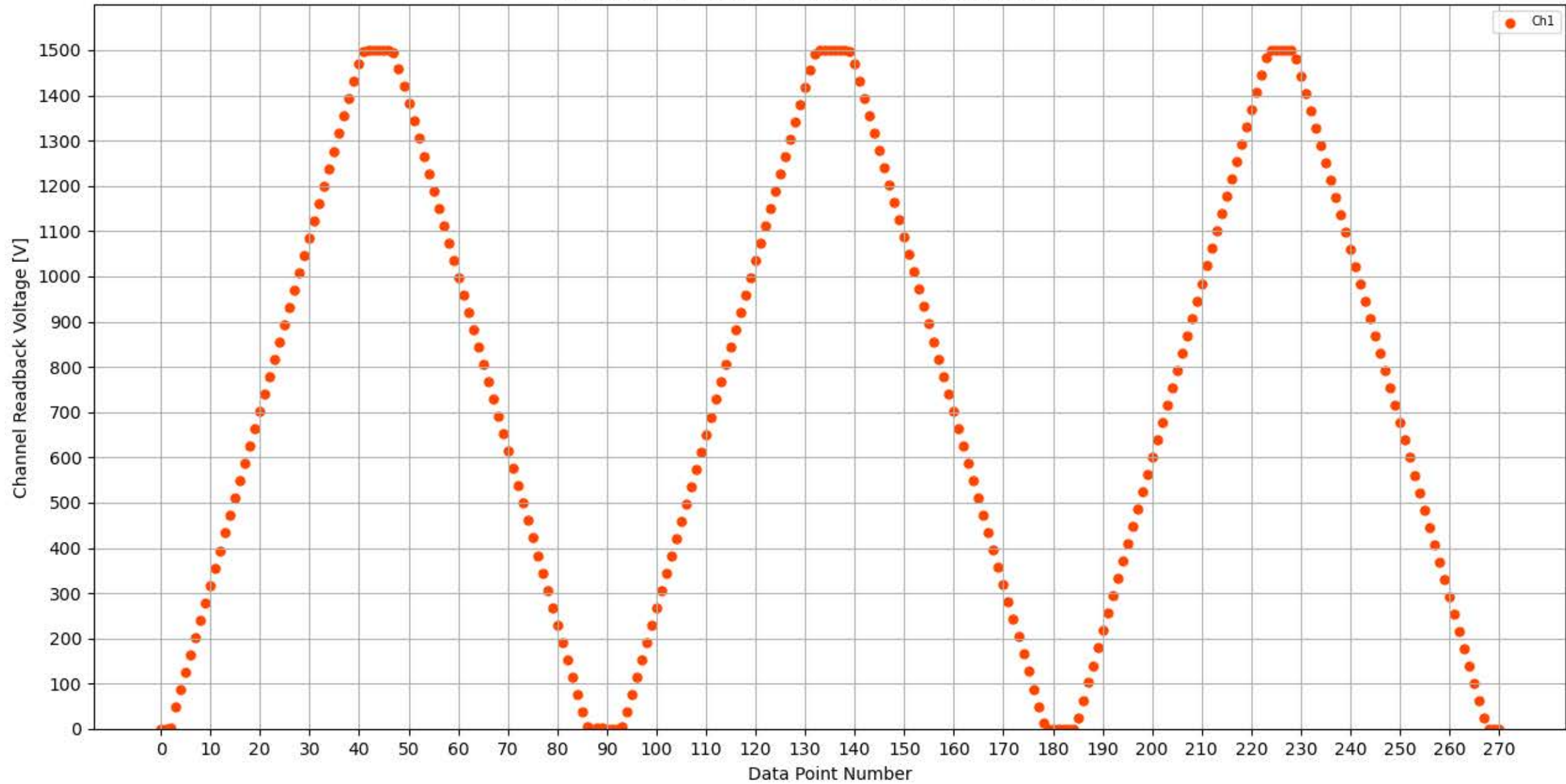
Voltage Ramp Test (Python) Bd #313, Slot #8, Ch #1
