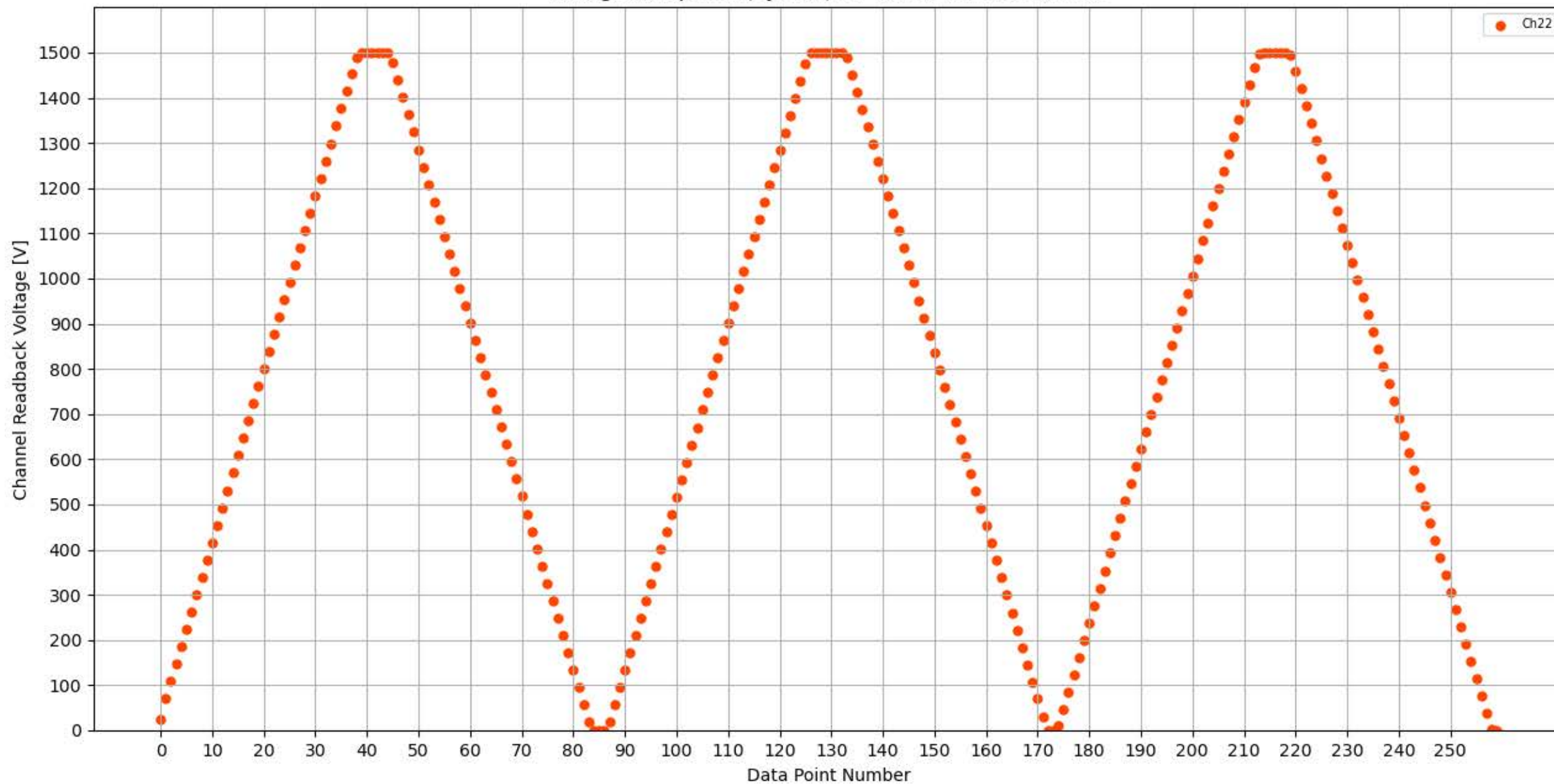
Voltage Ramp Test (Python) Bd #313, Slot #8, Ch #22
