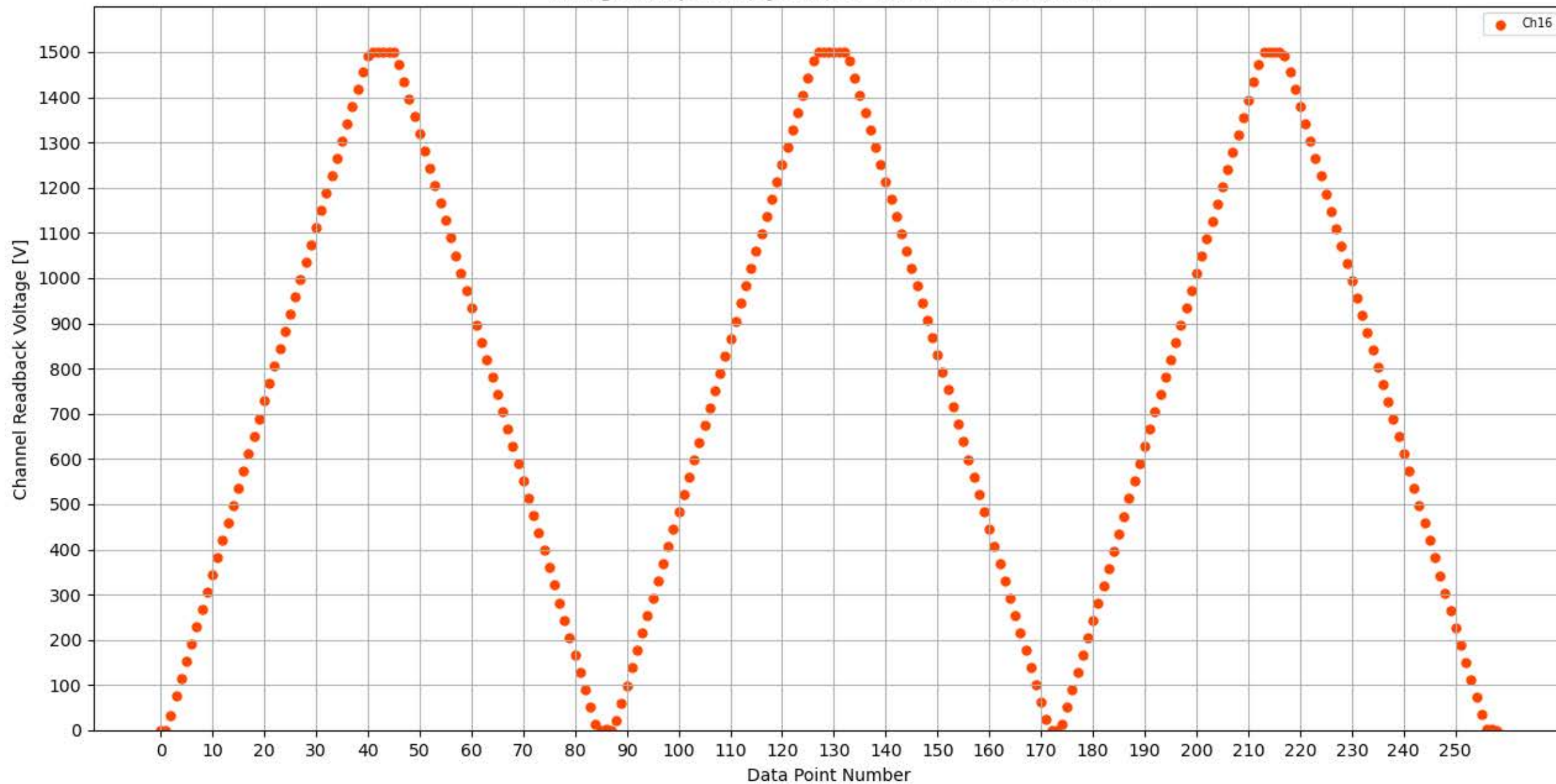
Voltage Ramp Test (Python) Bd #313, Slot #8, Ch #16
