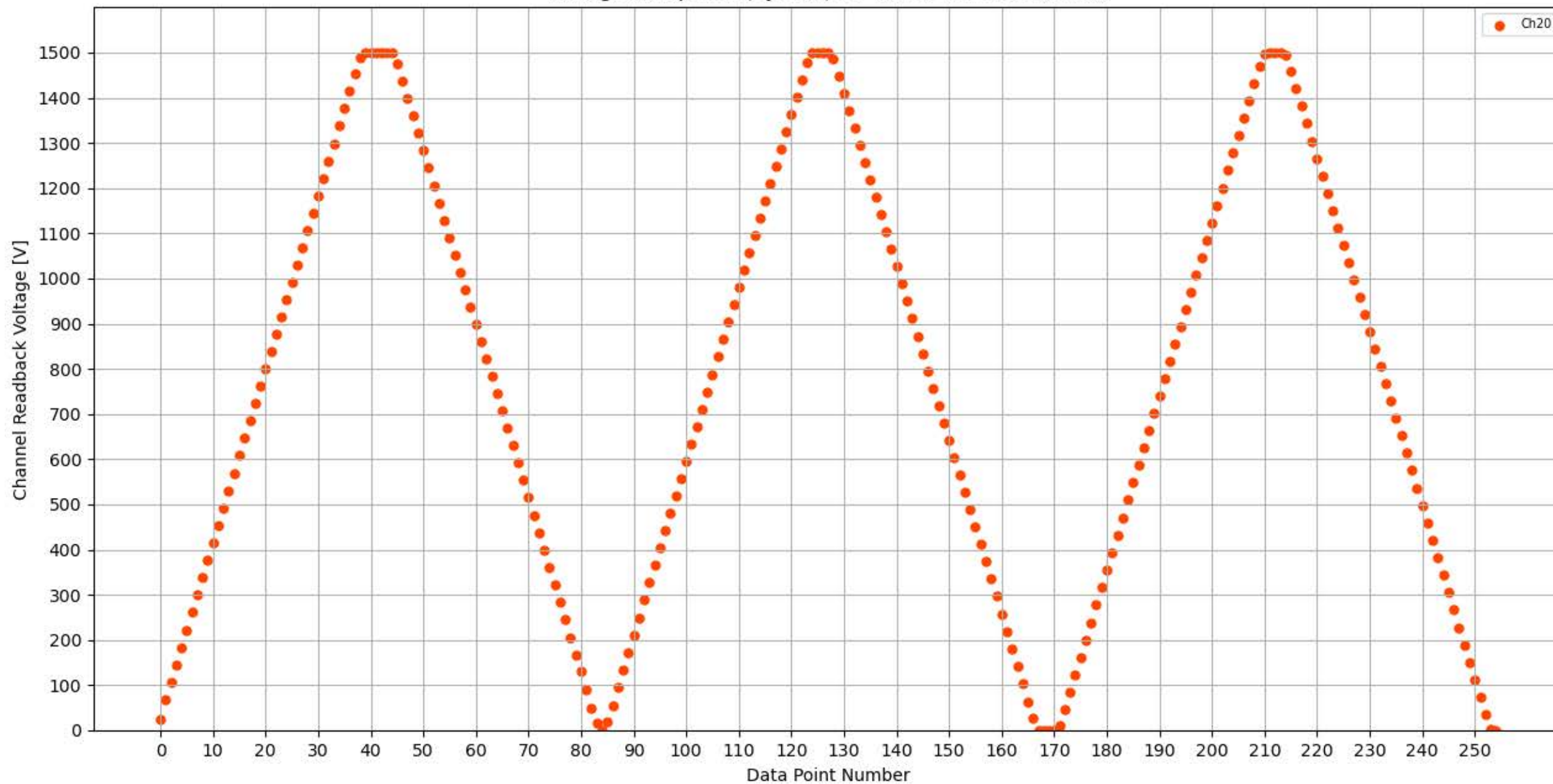
Voltage Ramp Test (Python) Bd #313, Slot #8, Ch #20
