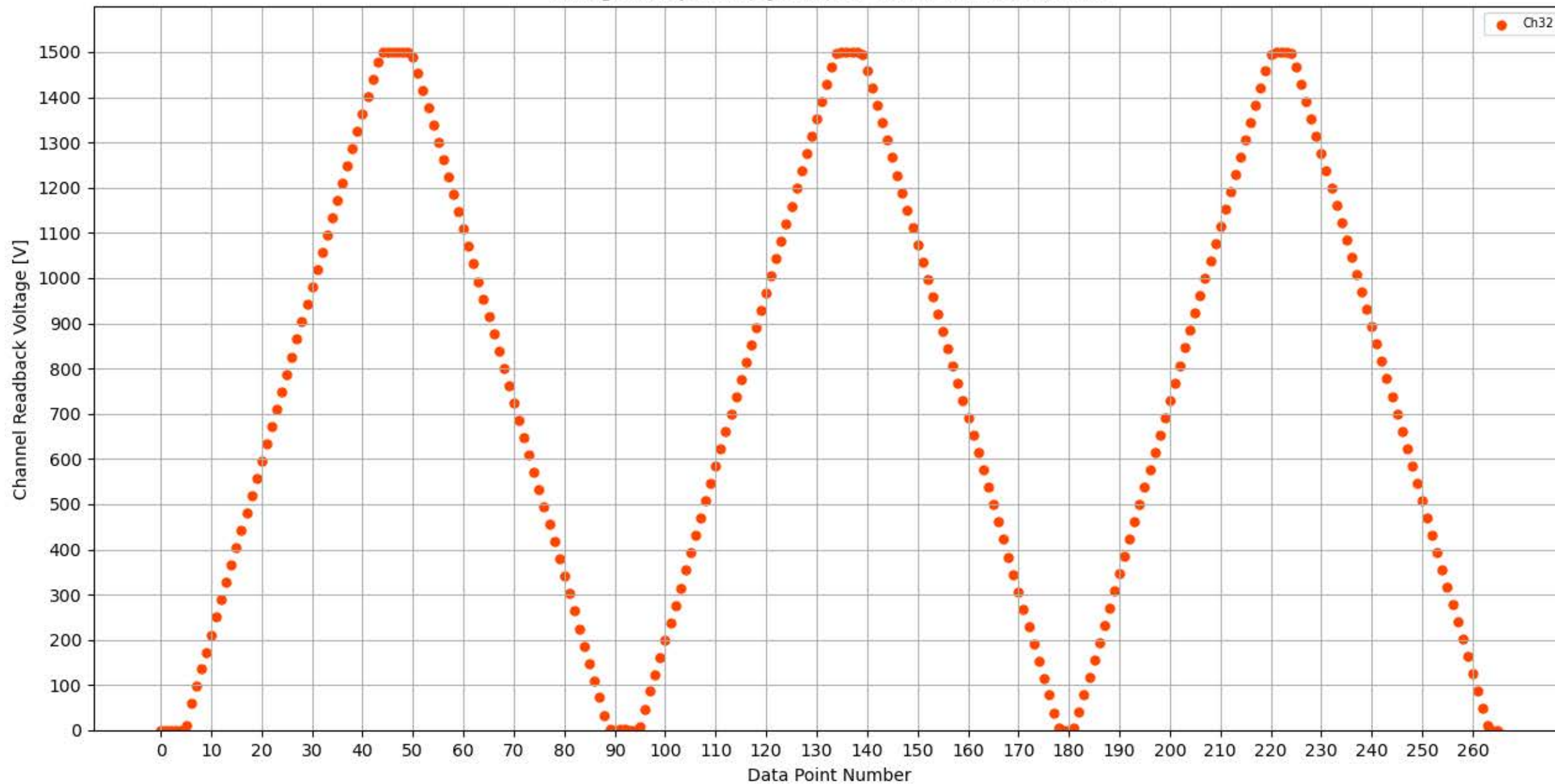
Voltage Ramp Test (Python) Bd #313, Slot #8, Ch #32
