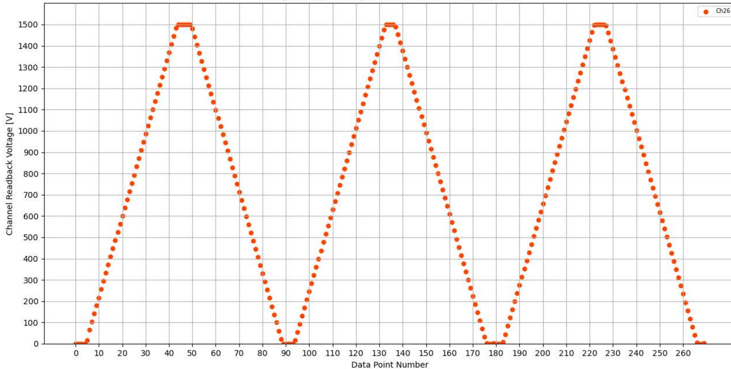
Voltage Ramp Test (Python) Bd #313, Slot #8, Ch #26
