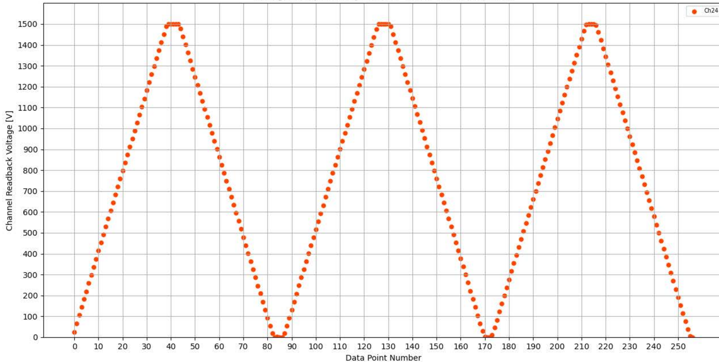
Voltage Ramp Test (Python) Bd #313, Slot #8, Ch #24
