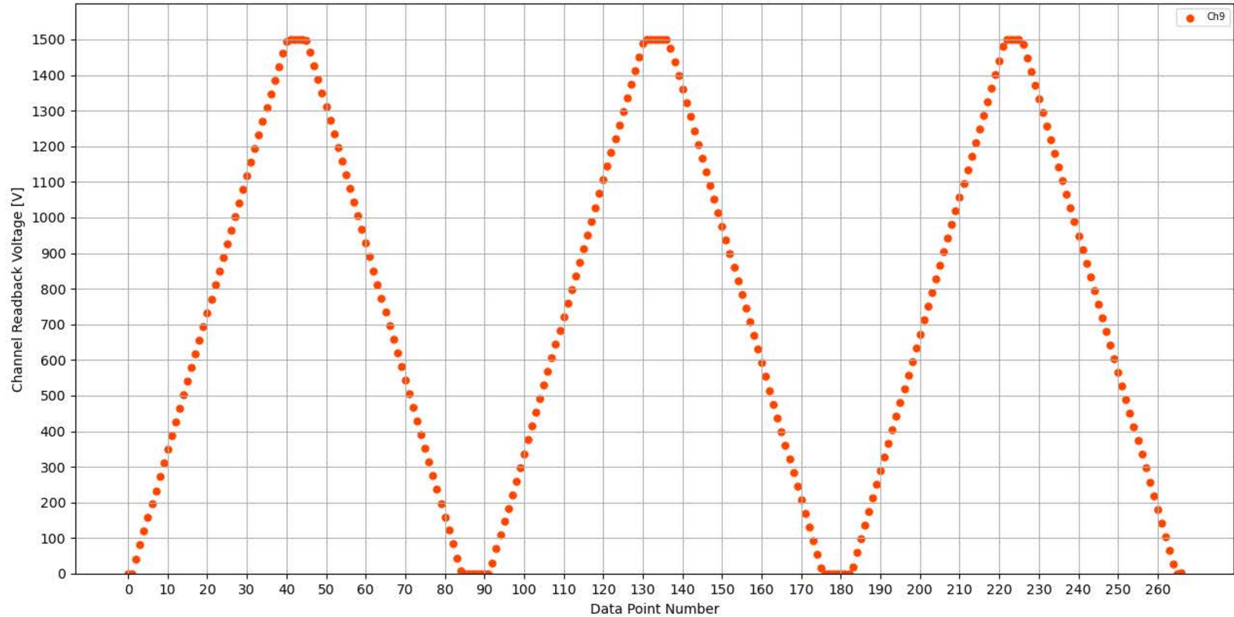
Voltage Ramp Test (Python) Bd #313, Slot #8, Ch #9
