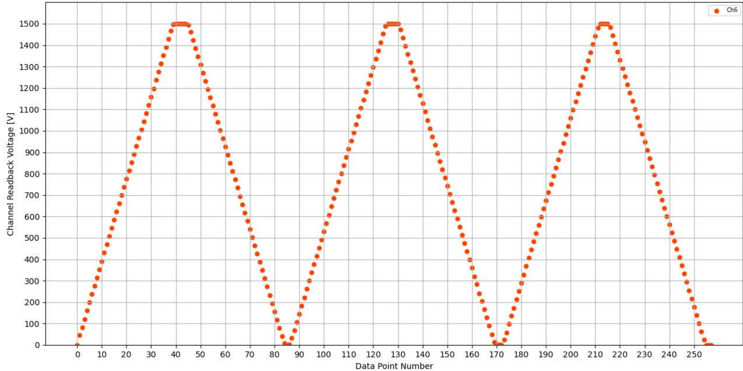
Voltage Ramp Test (Python) Bd #313, Slot #8, Ch #6
