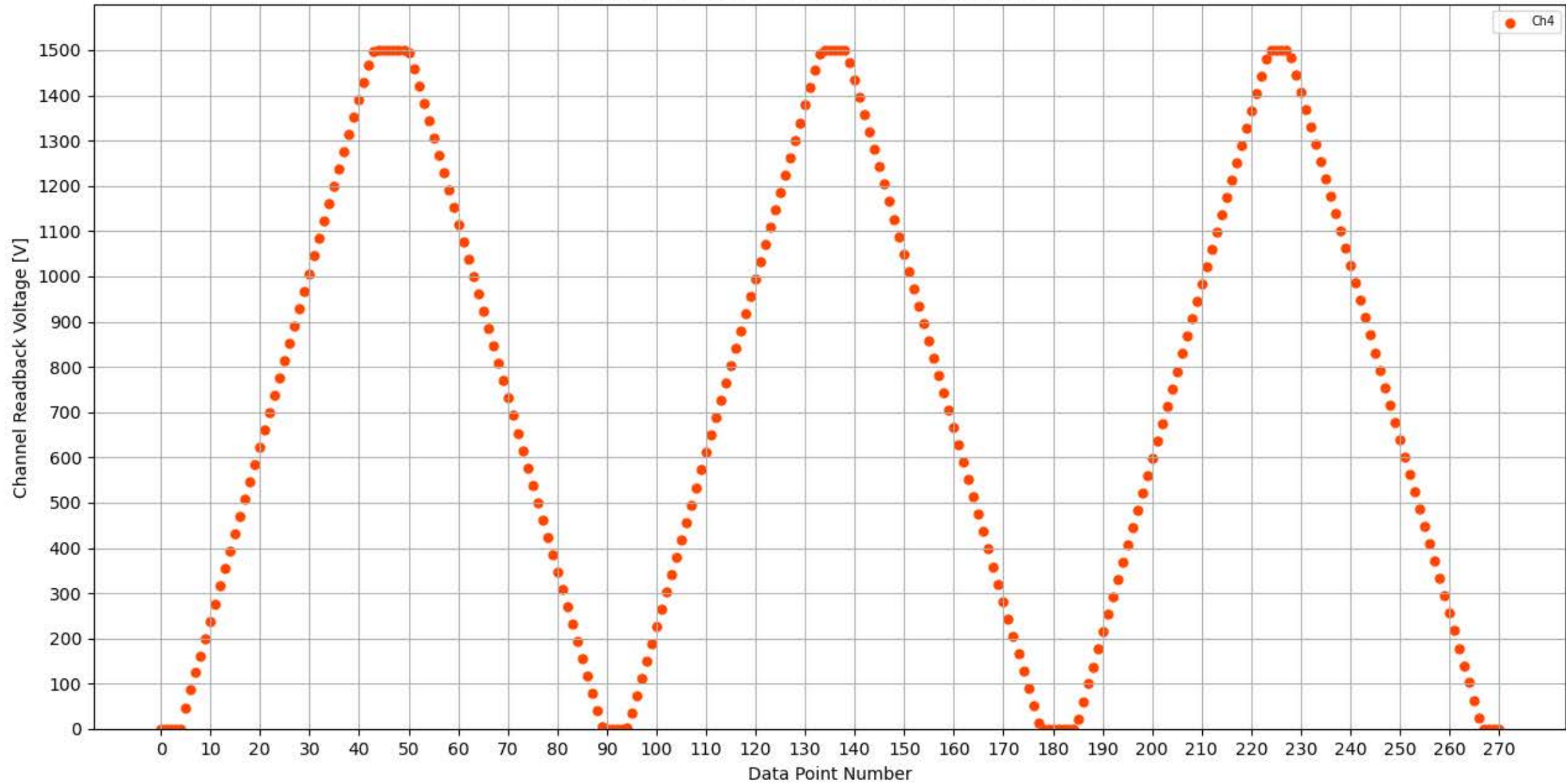
Voltage Ramp Test (Python) Bd #313, Slot #8, Ch #4
