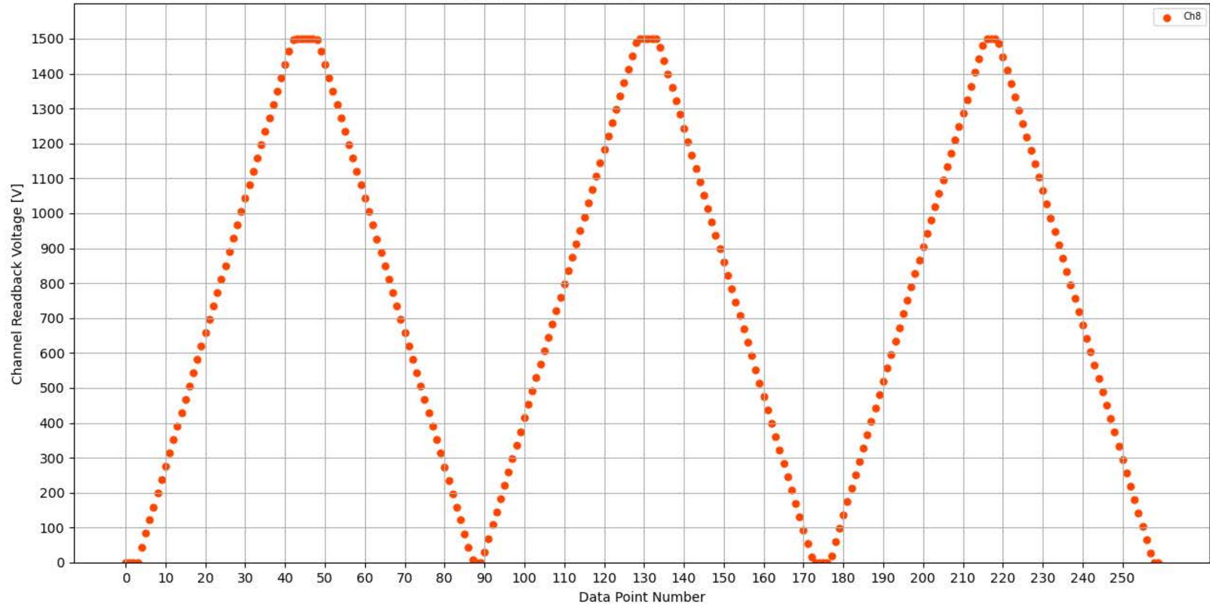
Voltage Ramp Test (Python) Bd #313, Slot #8, Ch #8
