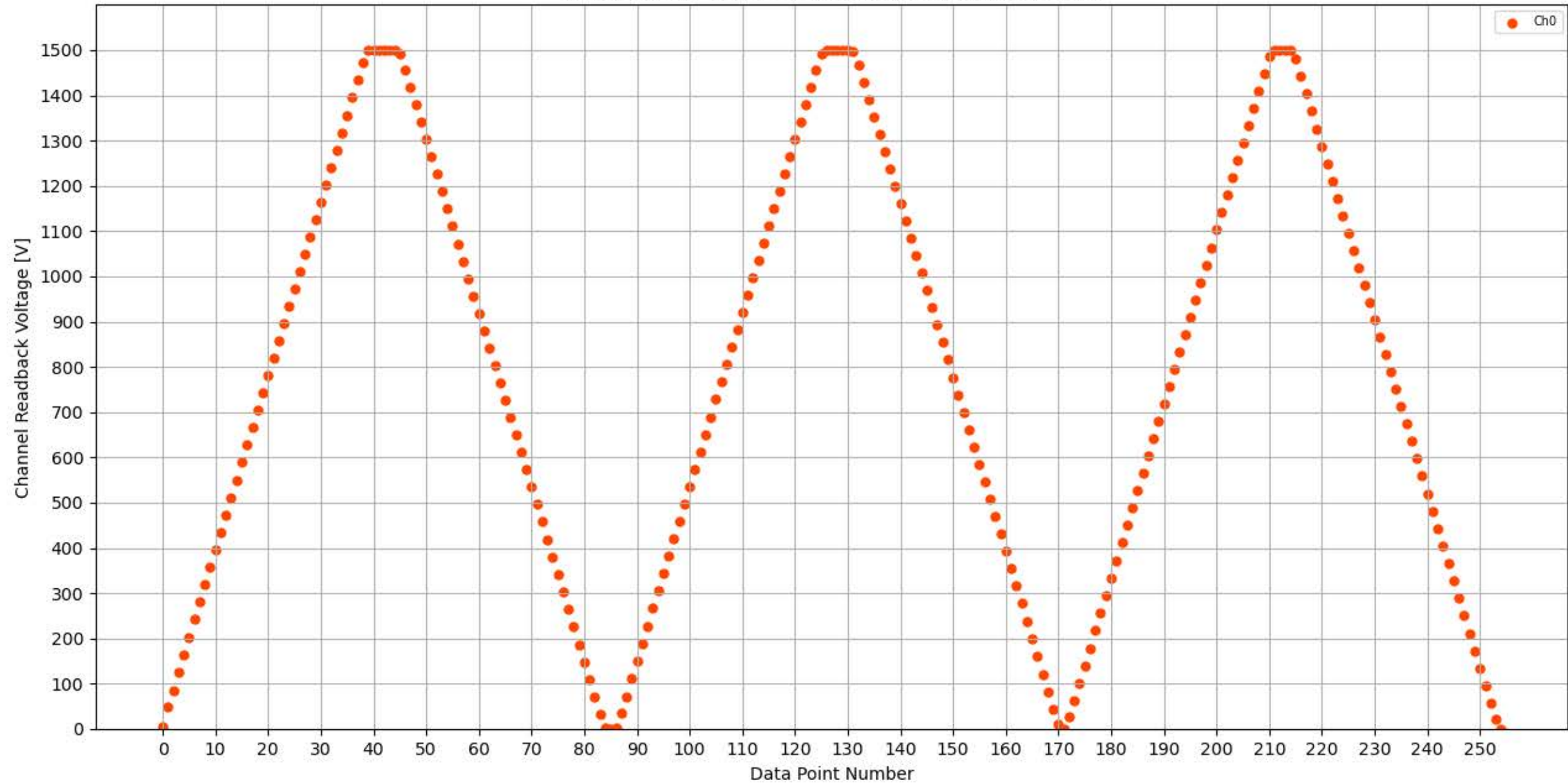
Voltage Ramp Test (Python) Bd #313, Slot #8, Ch #0
