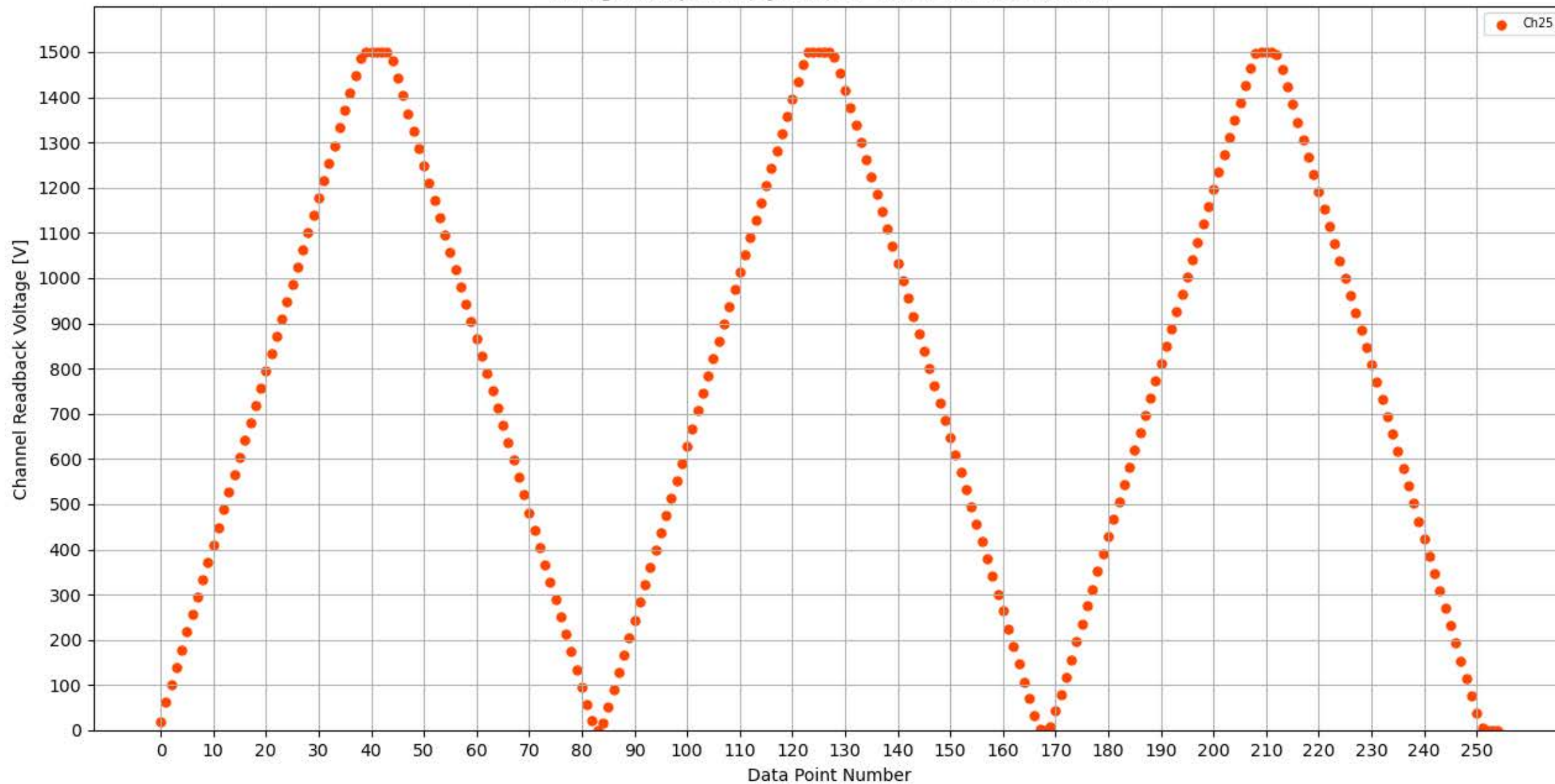
Voltage Ramp Test (Python) Bd #313, Slot #8, Ch #25
