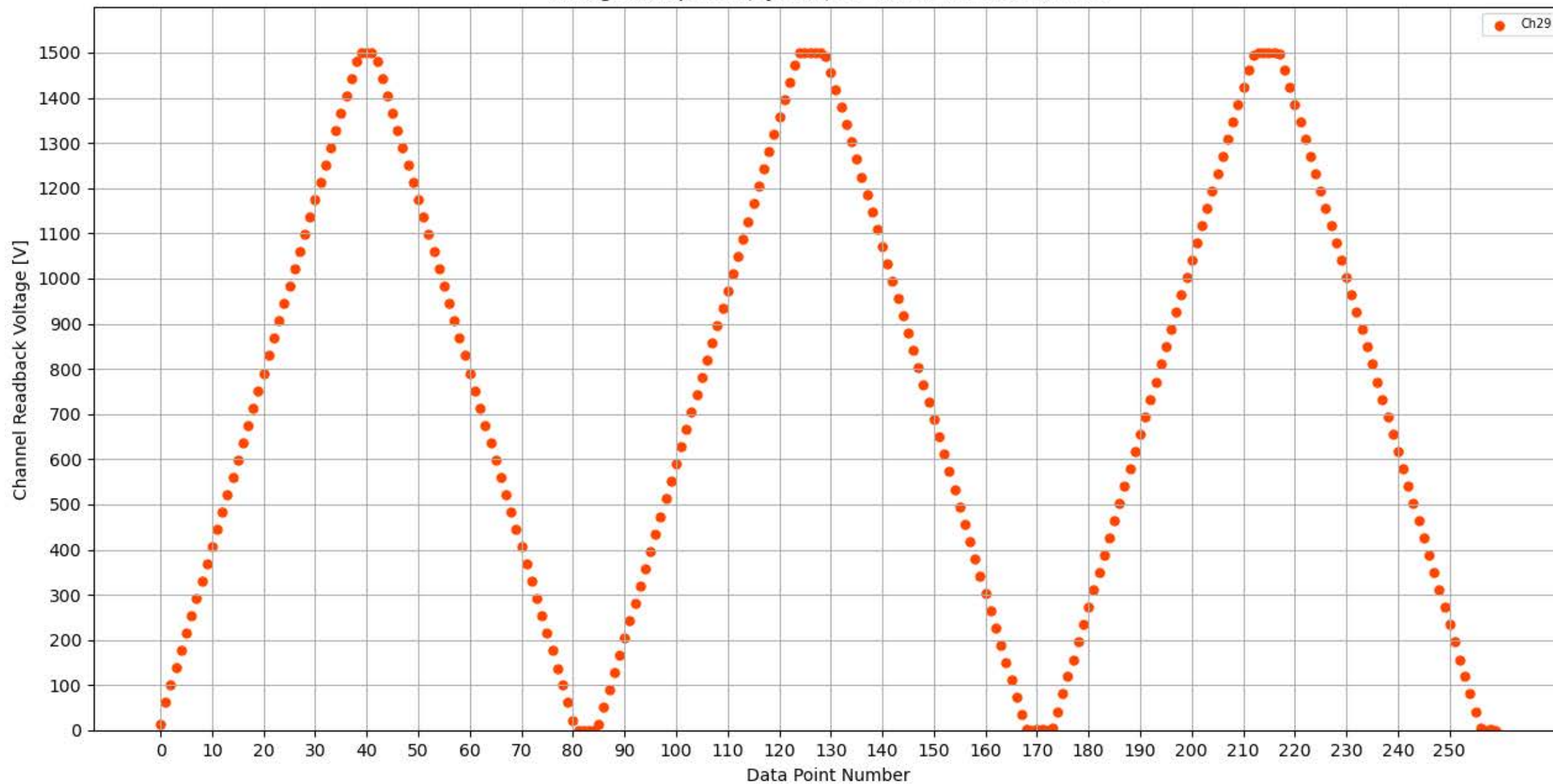
Voltage Ramp Test (Python) Bd #313, Slot #8, Ch #29
