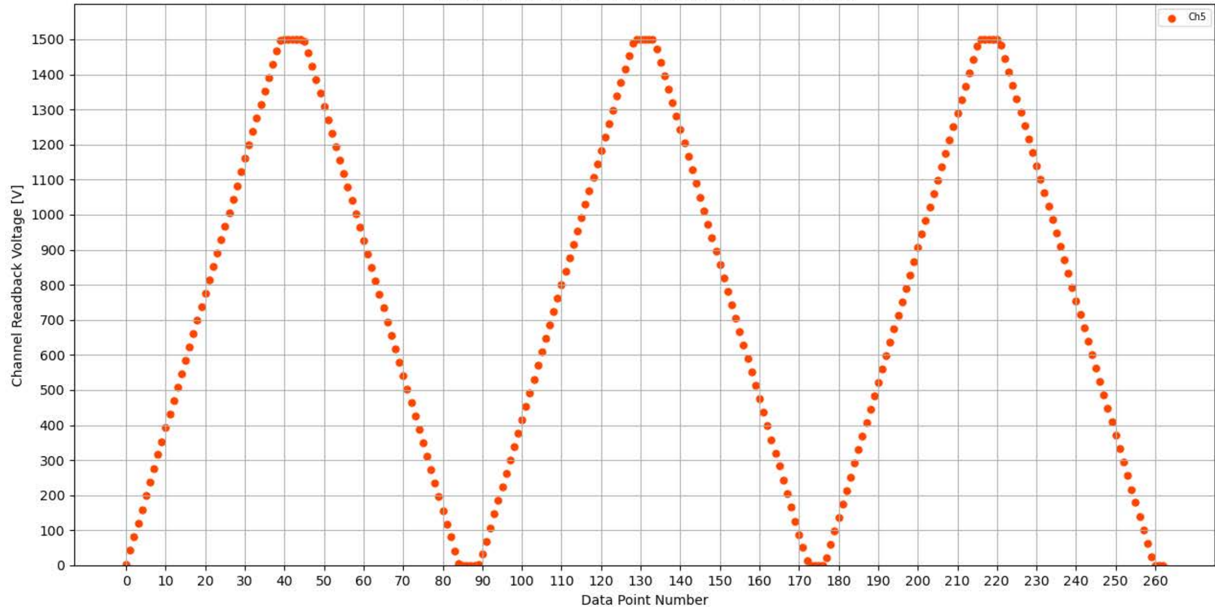
Voltage Ramp Test (Python) Bd #313, Slot #8, Ch #5
