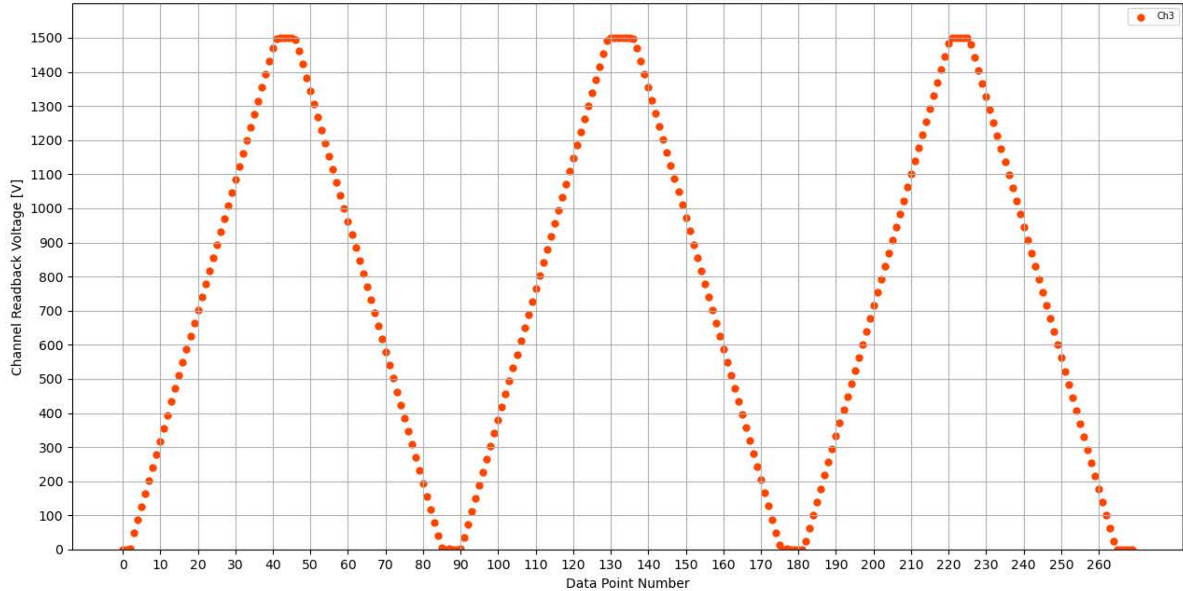
Voltage Ramp Test (Python) Bd #313, Slot #8, Ch #3
