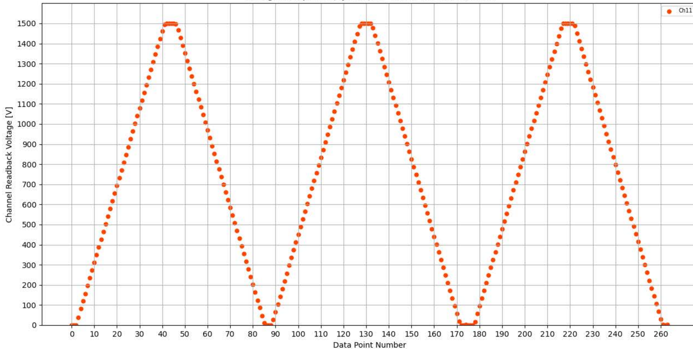
Voltage Ramp Test (Python) Bd #313, Slot #8, Ch #11
