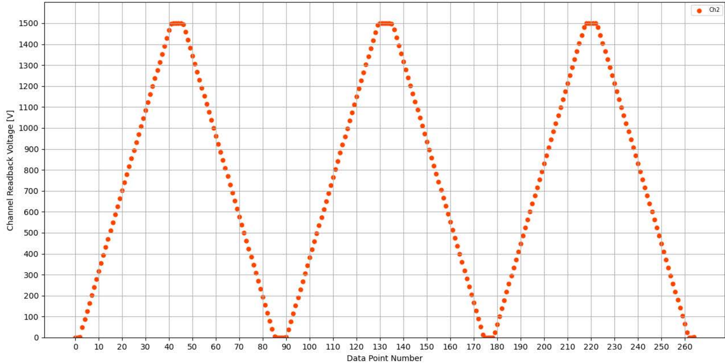
Voltage Ramp Test (Python) Bd #313, Slot #8, Ch #2
