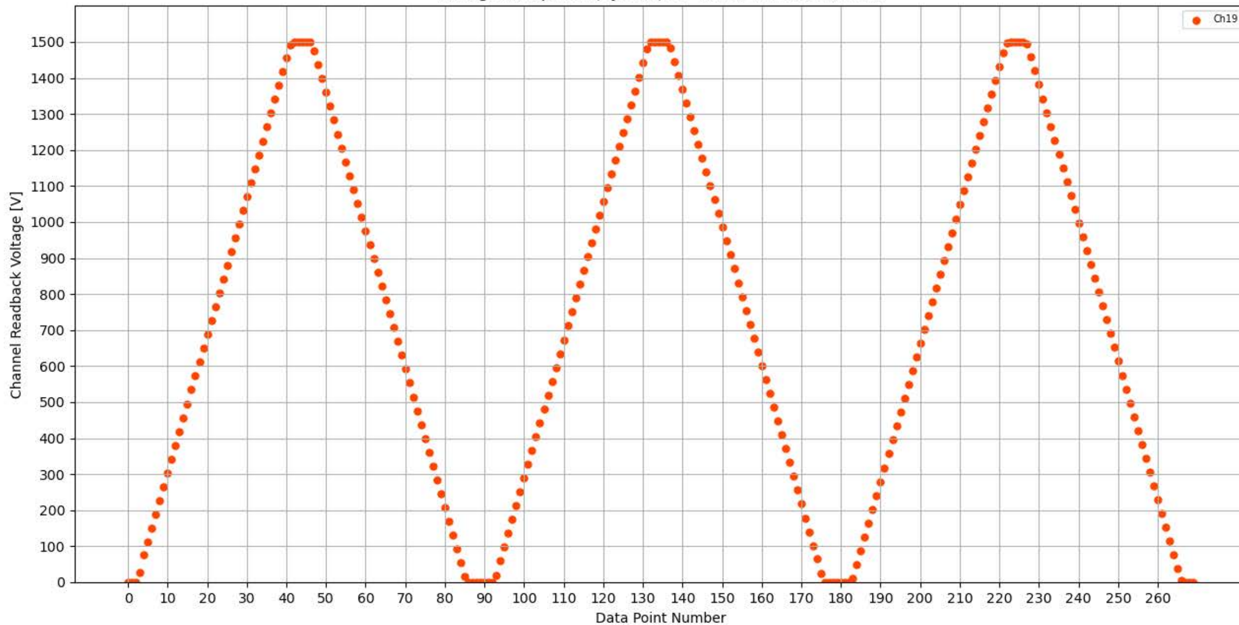
Voltage Ramp Test (Python) Bd #313, Slot #8, Ch #19
