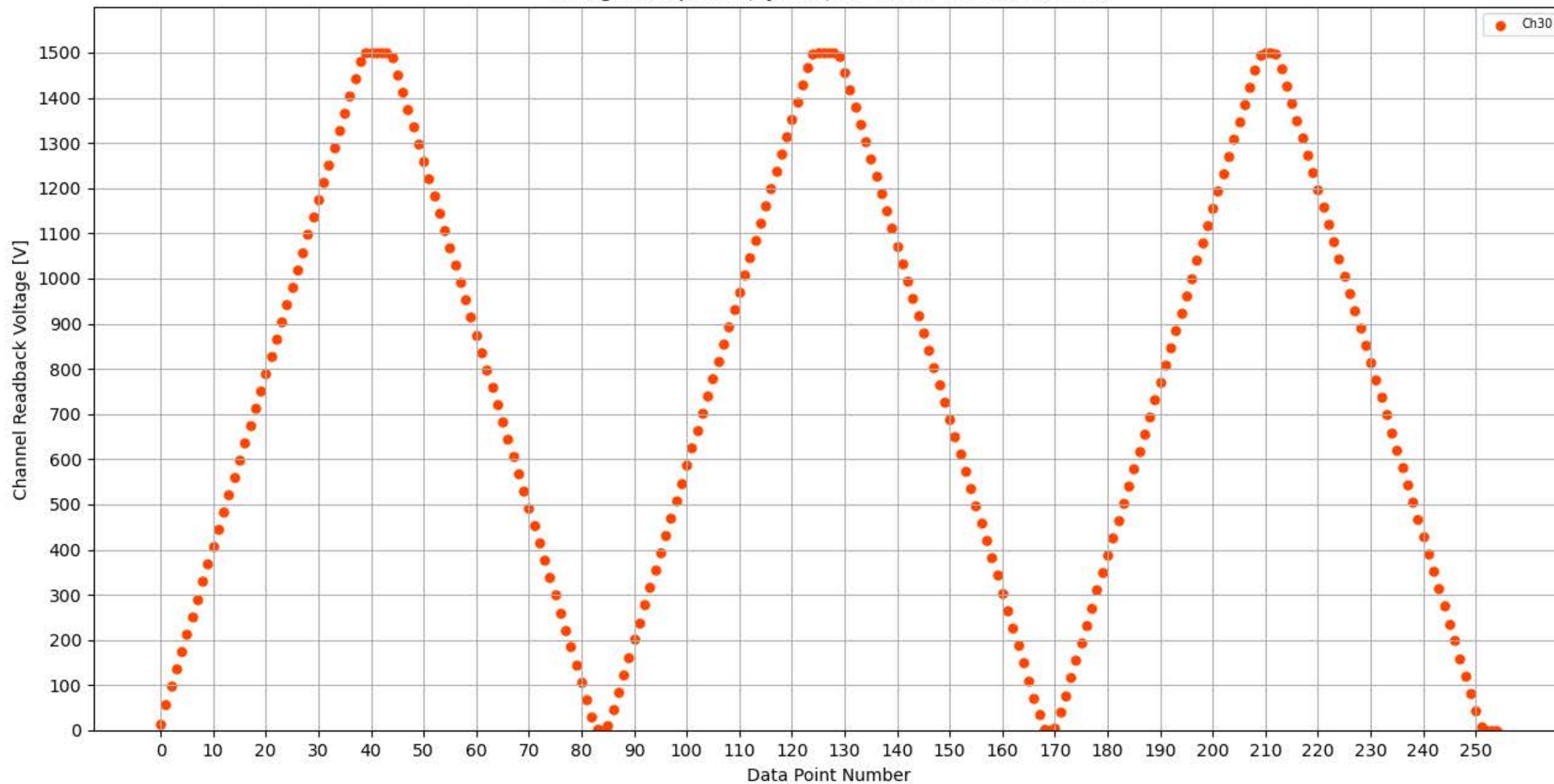
Voltage Ramp Test (Python) Bd #313, Slot #8, Ch #30
