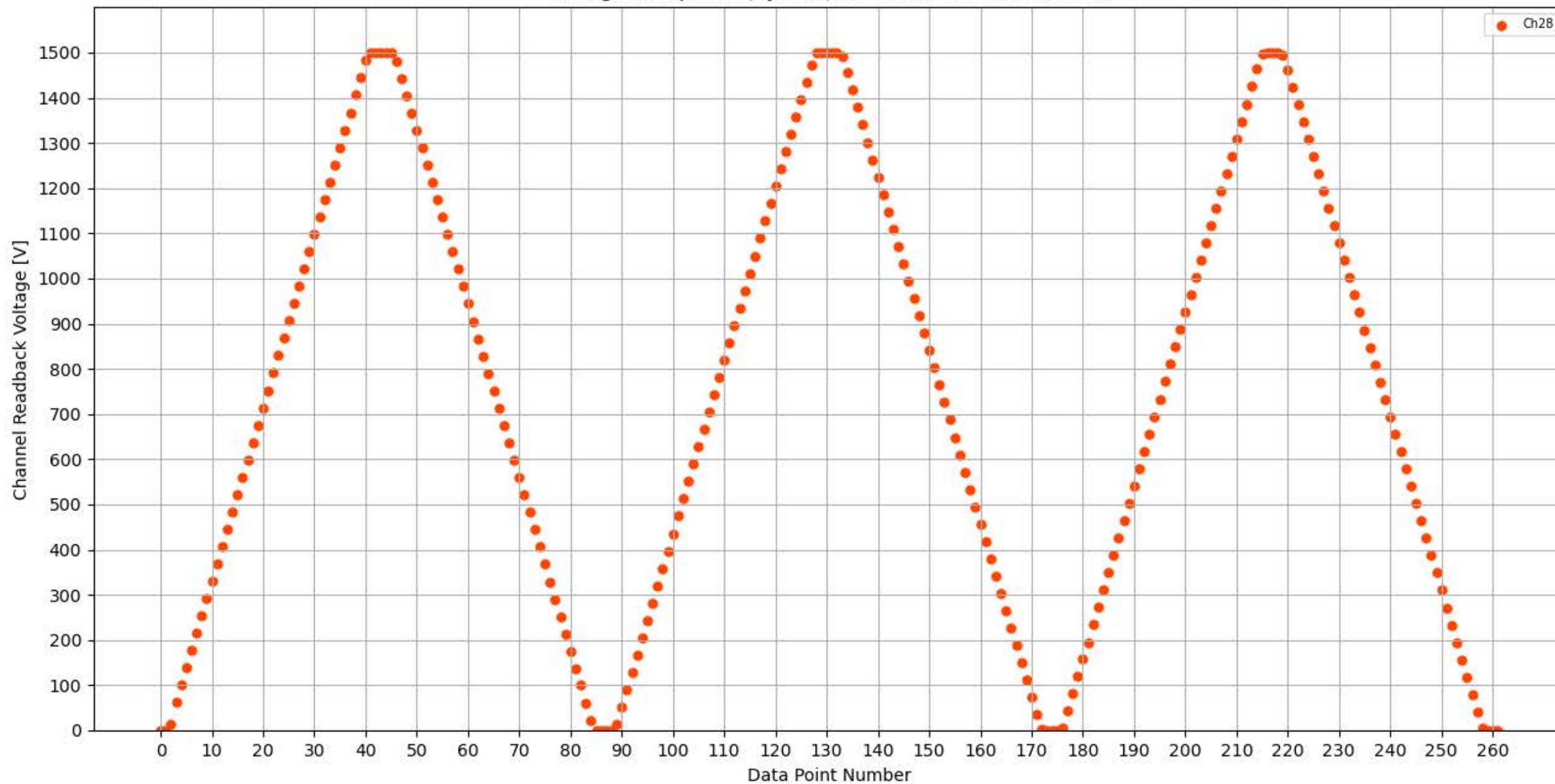
Voltage Ramp Test (Python) Bd #313, Slot #8, Ch #28
