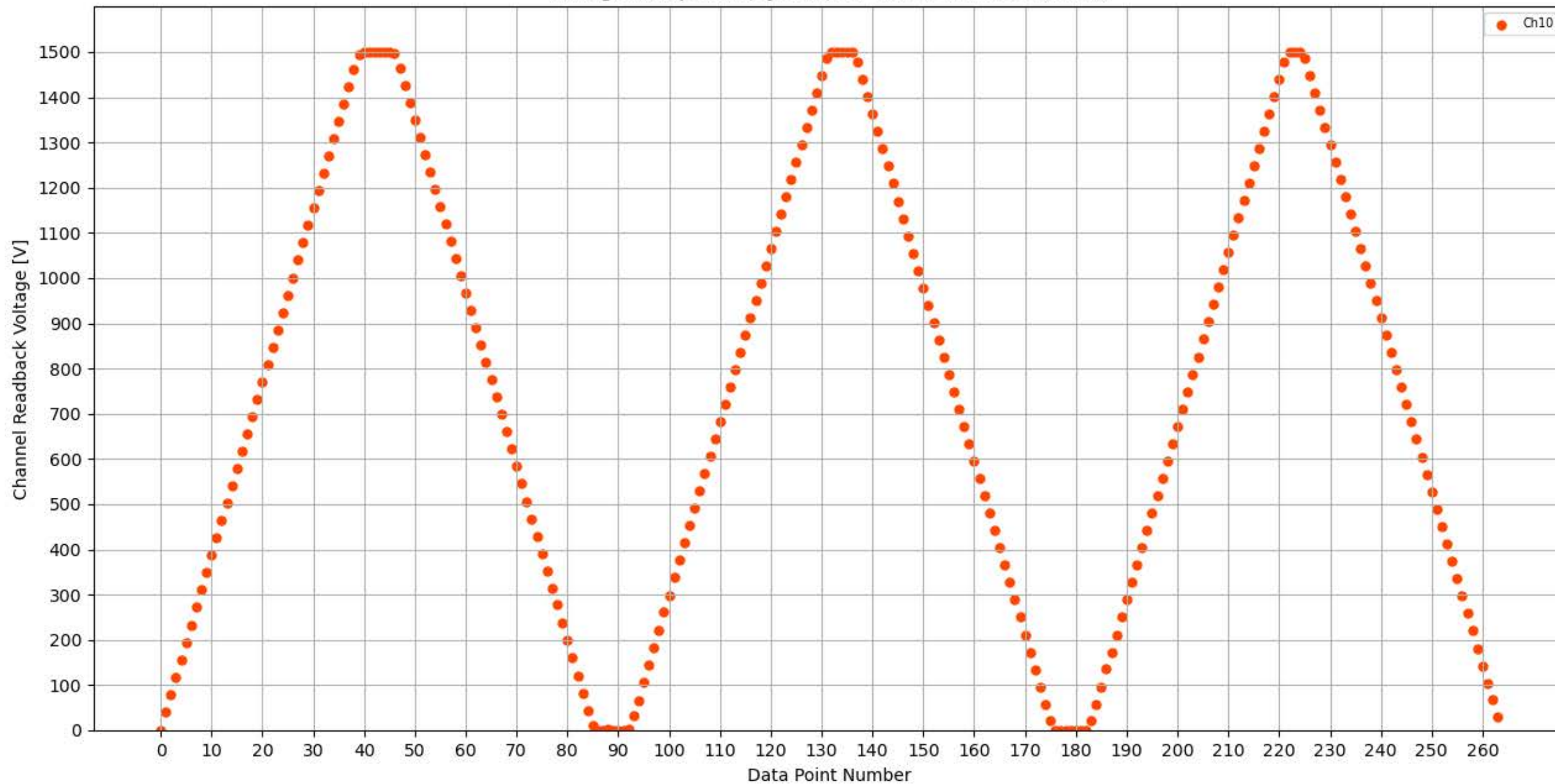
Voltage Ramp Test (Python) Bd #313, Slot #8, Ch #10
