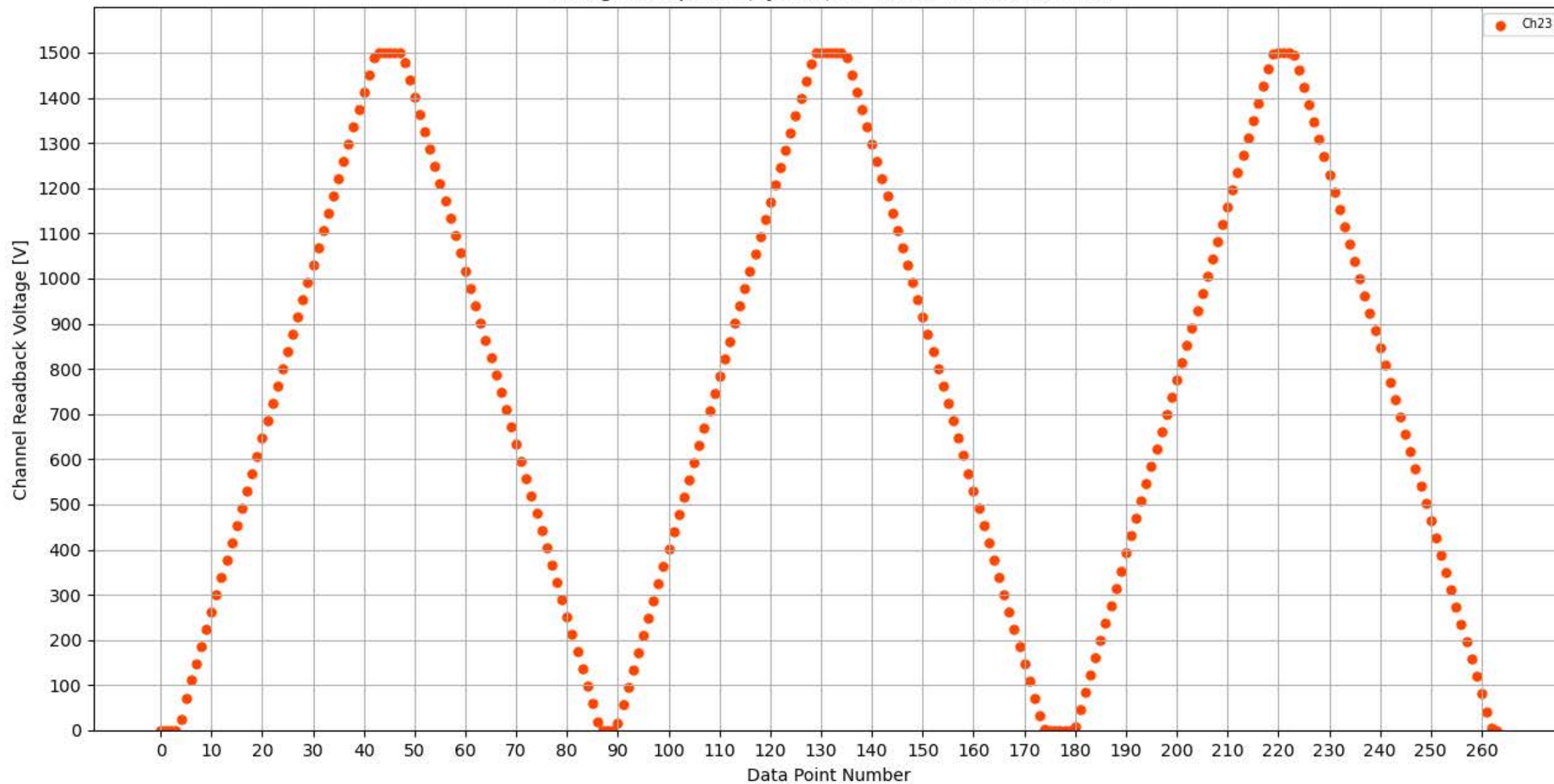
Voltage Ramp Test (Python) Bd #313, Slot #8, Ch #23
